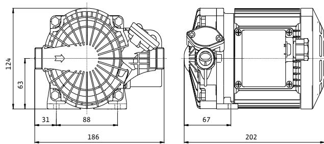
PB-S125EA
