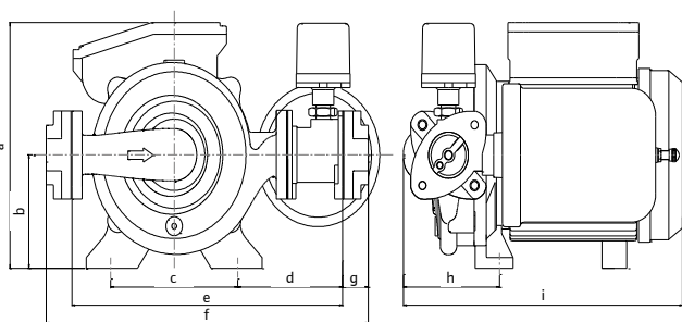
PB-250SEA, PB-401SEA
