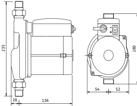
PB-088EA
